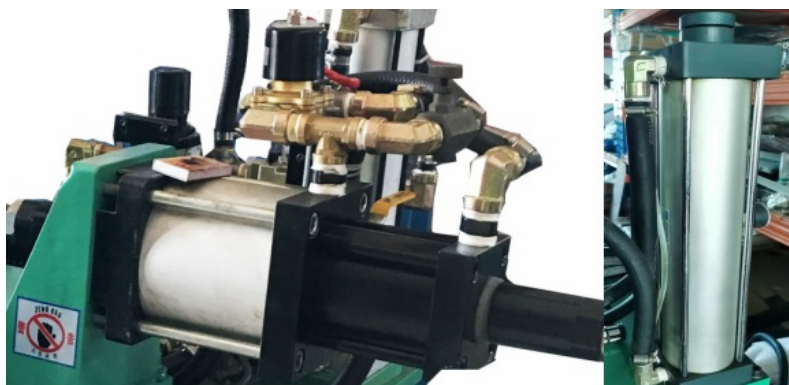
Welding sample display
